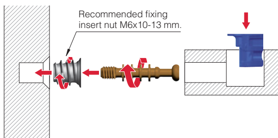
INSTALLATION WITH M6 DOWEL
