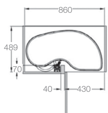
Example: Cabinet 900 Right version application
