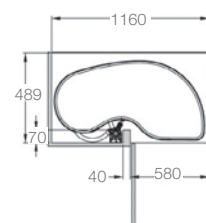
Example: Cabinet 1200 Right version application
